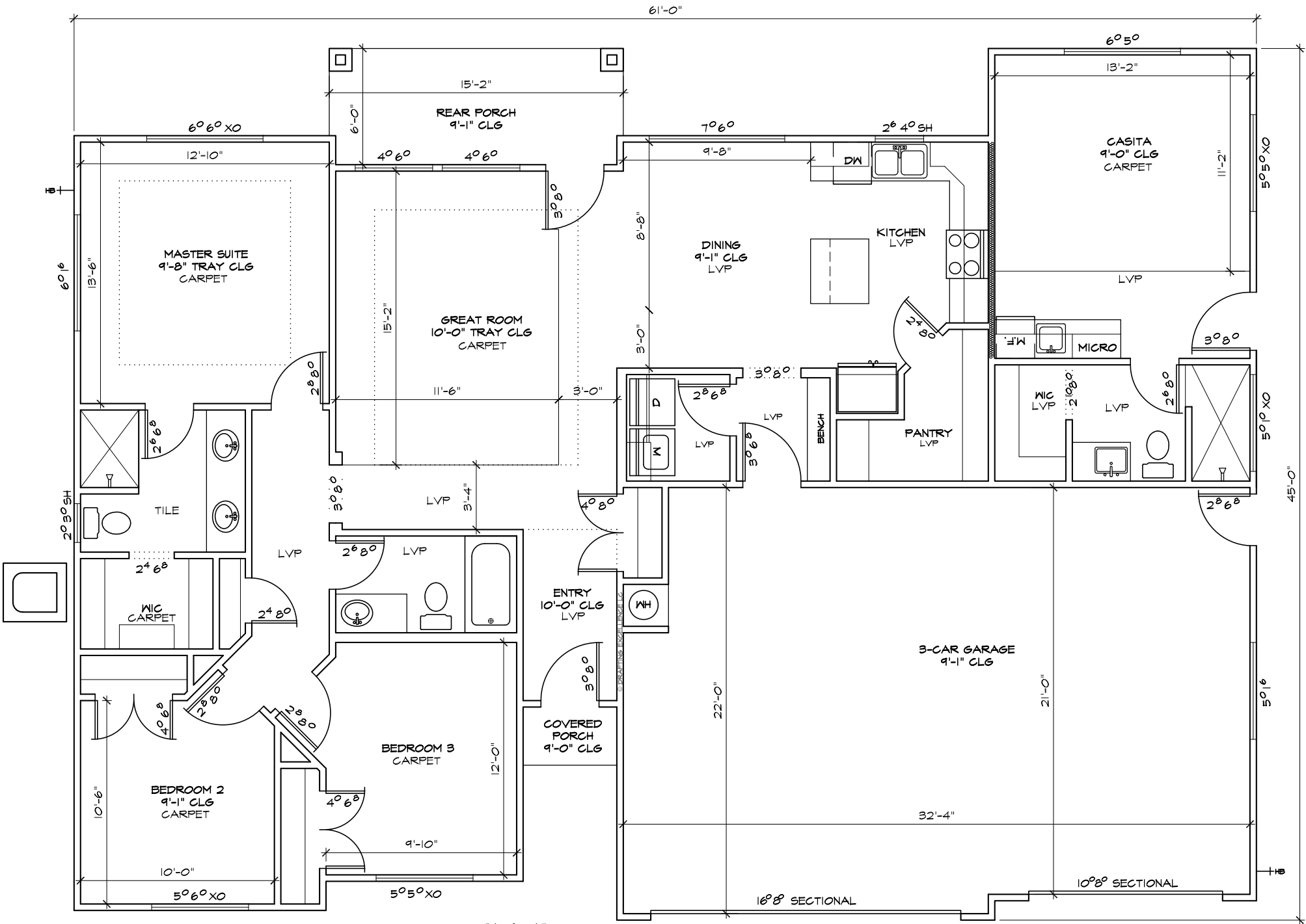
SLATE 1,709 SQ FT © DRAFTING EXCELLENCE LC
