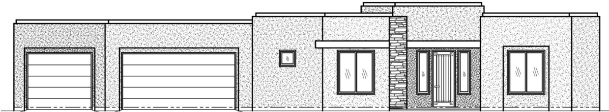
FRONT VIEW
